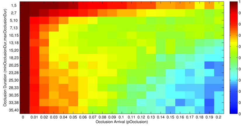
(a) Purity
