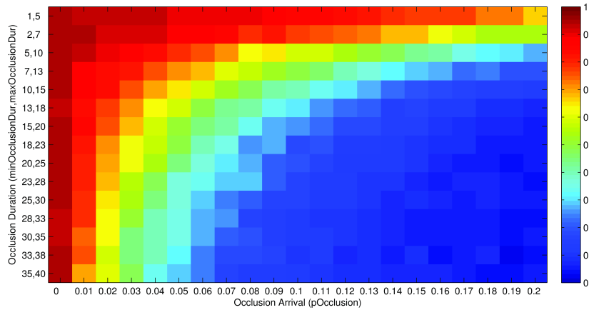
(b) Completeness
