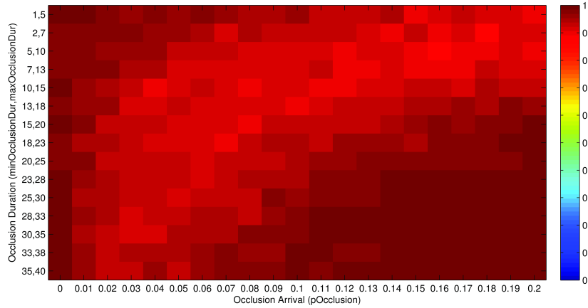
(a) Purity
